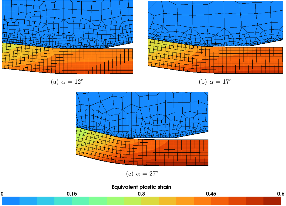
FIGURE 9: Equivalent plastic strain of the tube for three values of die angle, at the steady state (tube sinking case)
