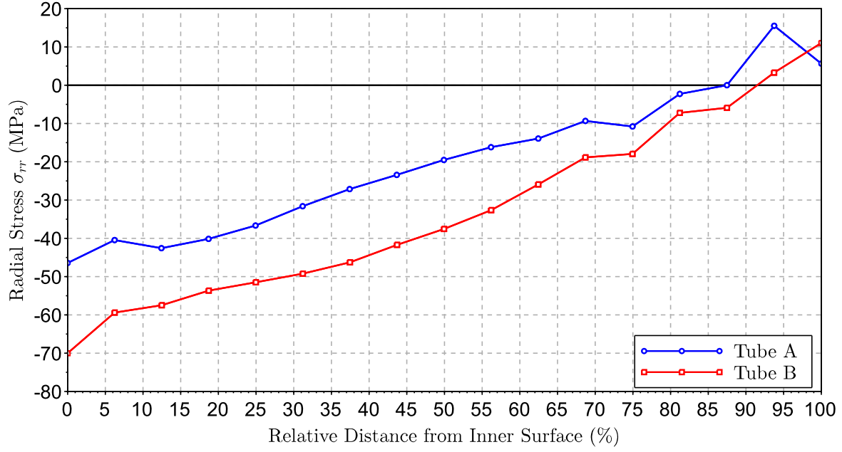
FIGURE 13: Repartition of radial stress before reeling operation
